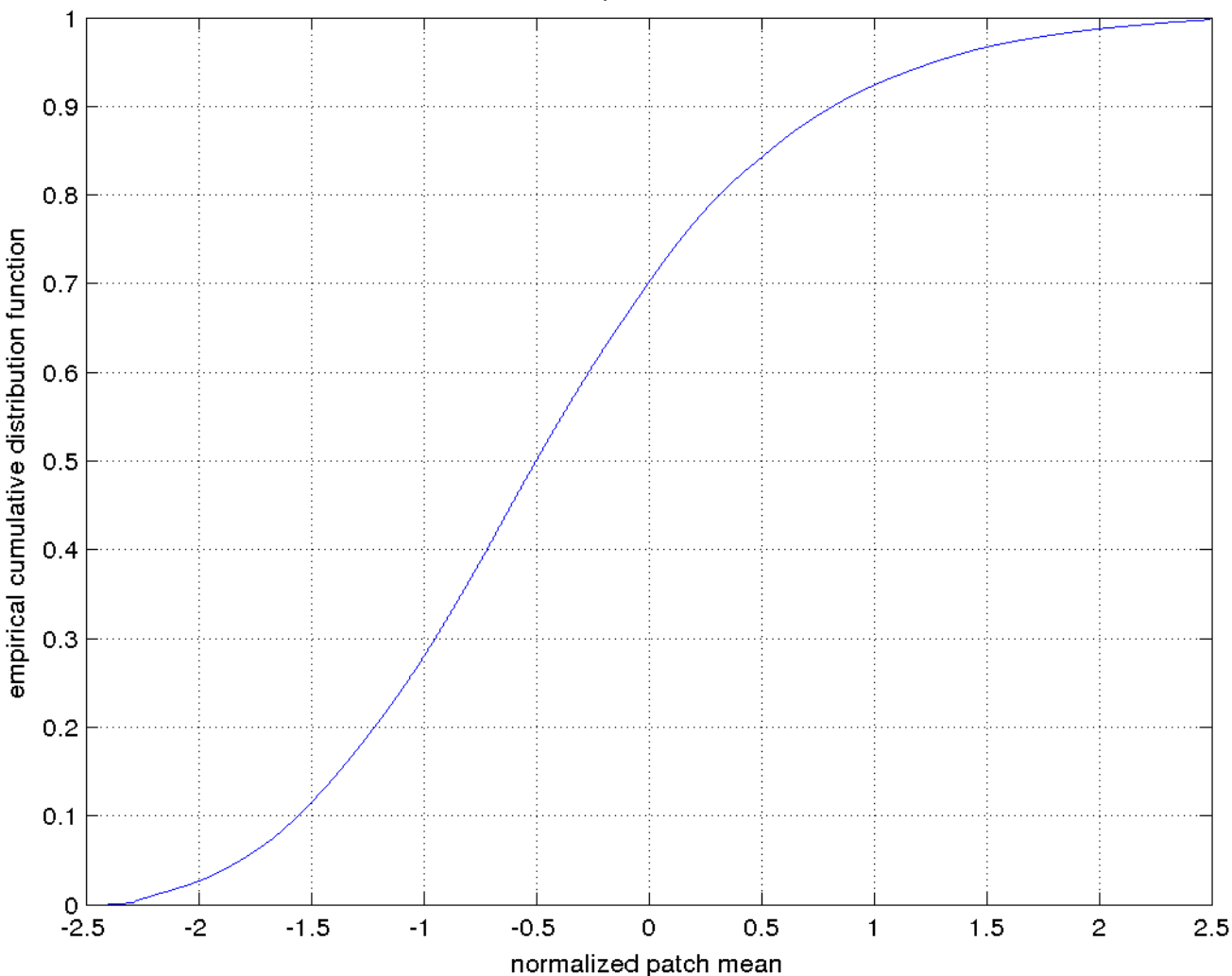
Empirical CDF
